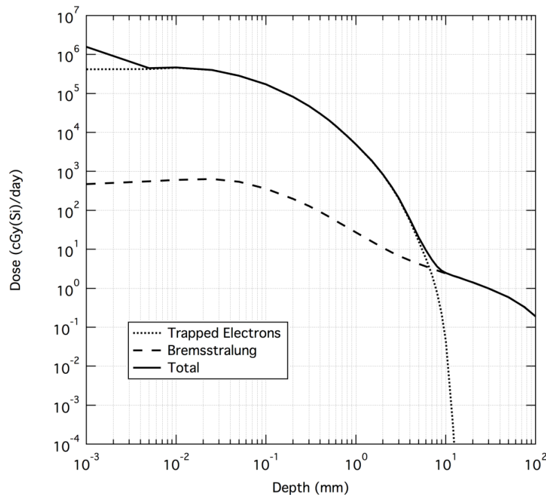
Figure 3.3.1.3-2. Daily Trapped Belts TID Inside Shielding
