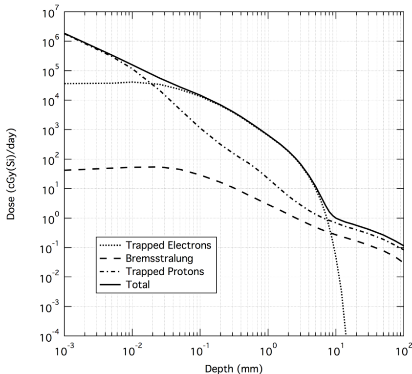
Figure 3.3.1.2.4-3. Daily Trapped Belts TID Inside Shielding
